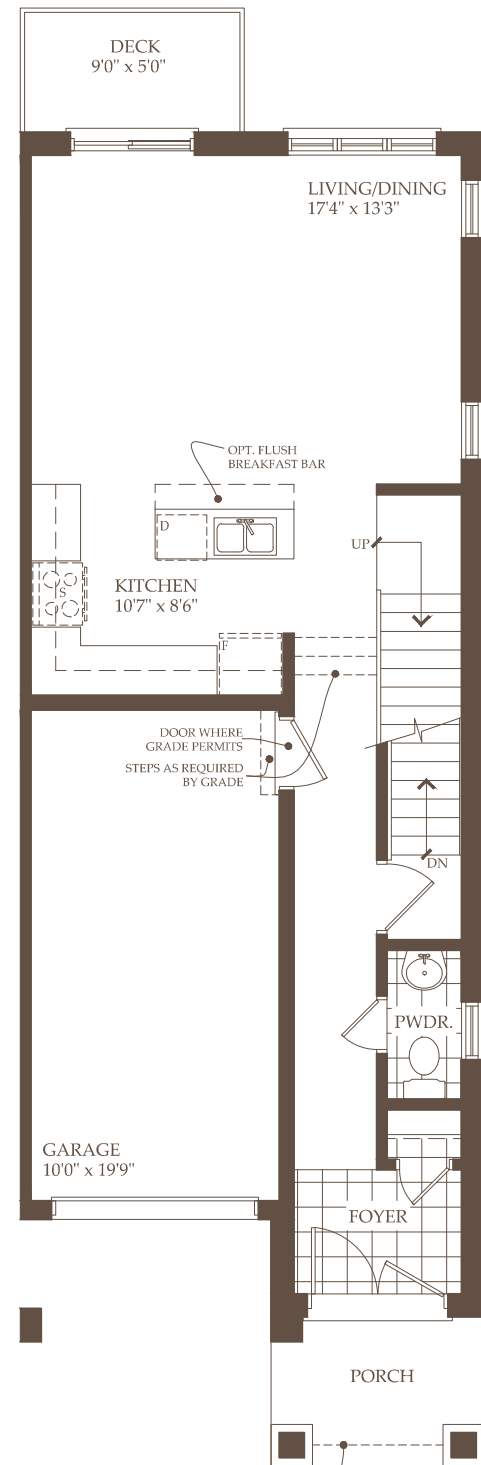
FIRST FLOOR
