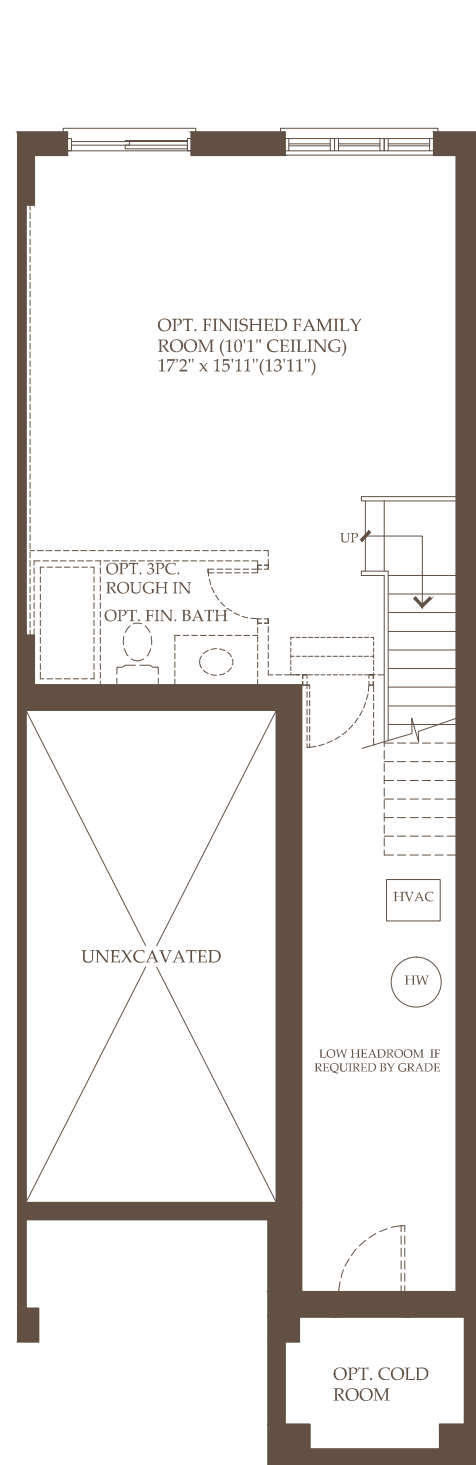
BASEMENT
