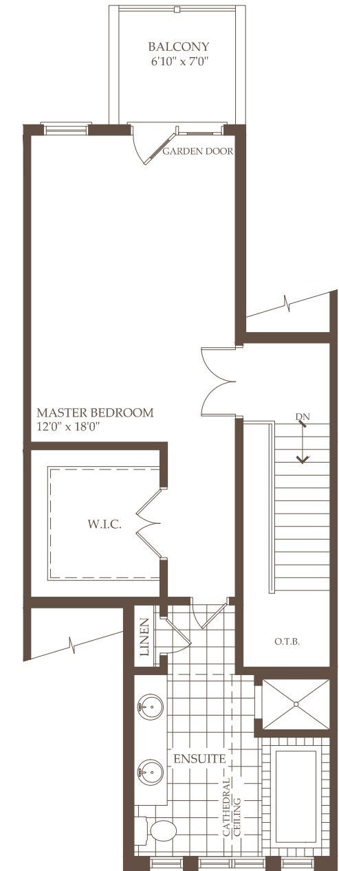
THIRD FLOOR
